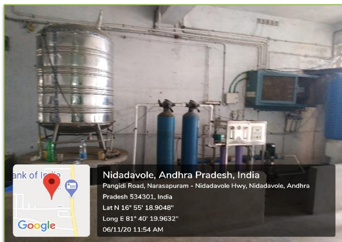
Figure 3: R.O. Water plant - Outlet is connected to garden
