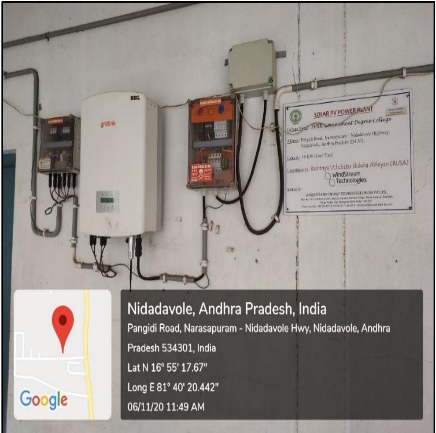
Figure 1 Solar PV system and Wheeling to grid
